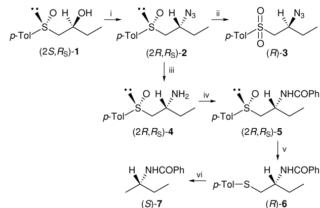
Scheme 1 Reagents, conditions and yields: i Method A: NaN 3 , Ph 3 P, CBr 4 (76%); Method B: HN 3 , Ph 3 P, DEAD (57%); ii, m -CPBA, 0 °C (96%); iii, HS[CH 2 ] 3 SH–NEt 3 (97%); iv, PhCO 2 H–DCC (72%); v, (CF 3 CO) 2 O–NaI (83%); Raney-Ni–H 2 , 60 °C (94%)
